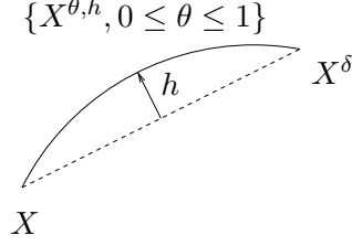
Figure 2: The graph of \theta \mapsto X^{\theta,h}
